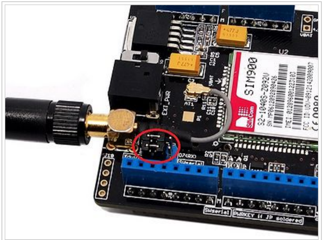
GPRS communicate with arduino by hardware serial
