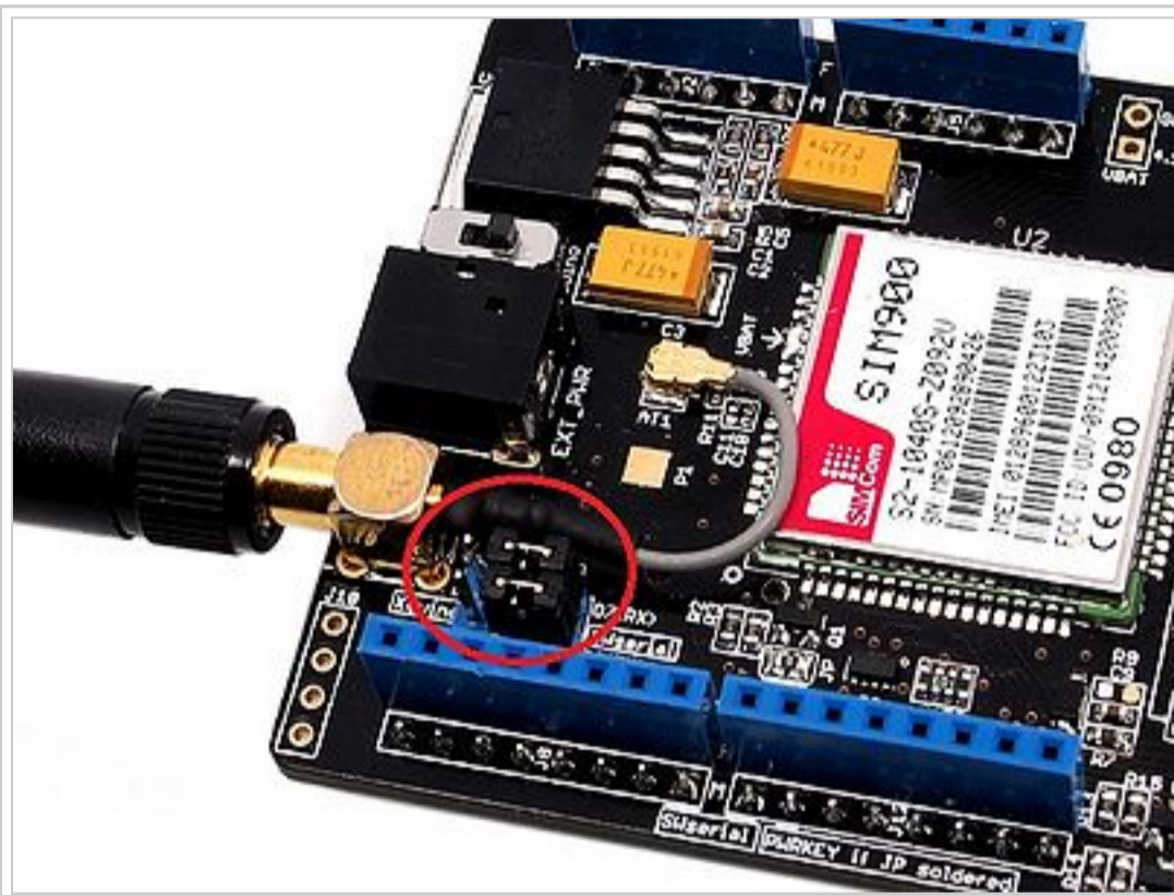
GPRS communicate with arduino by software serial
